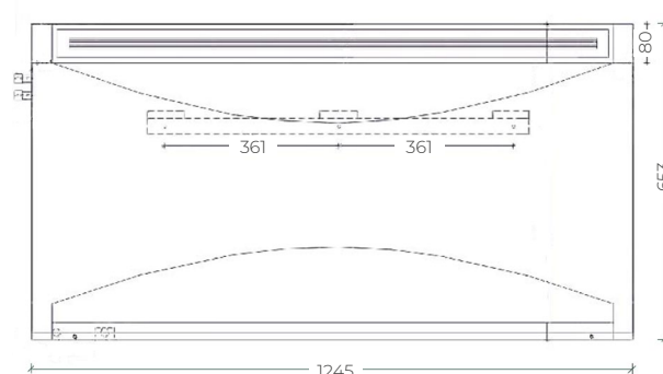
Diagrama DRY PLASTIK WAVE 500
