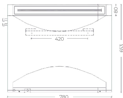
Diagrama DRY PLASTIK WAVE 300
